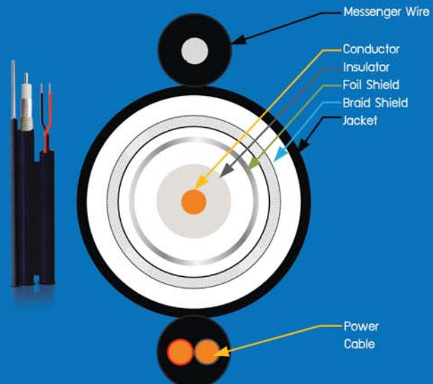
Structure: 3
