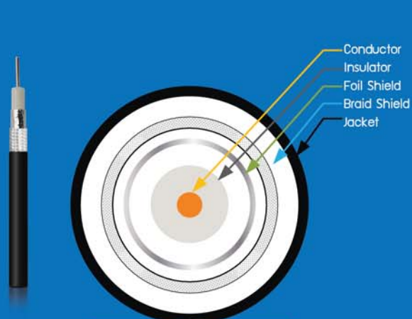
Structure: 1
