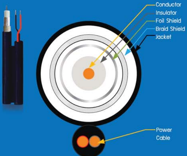
Structure: 3
