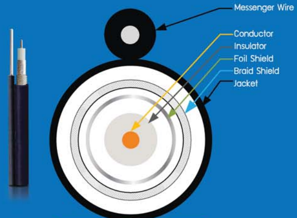
Structure: 2
