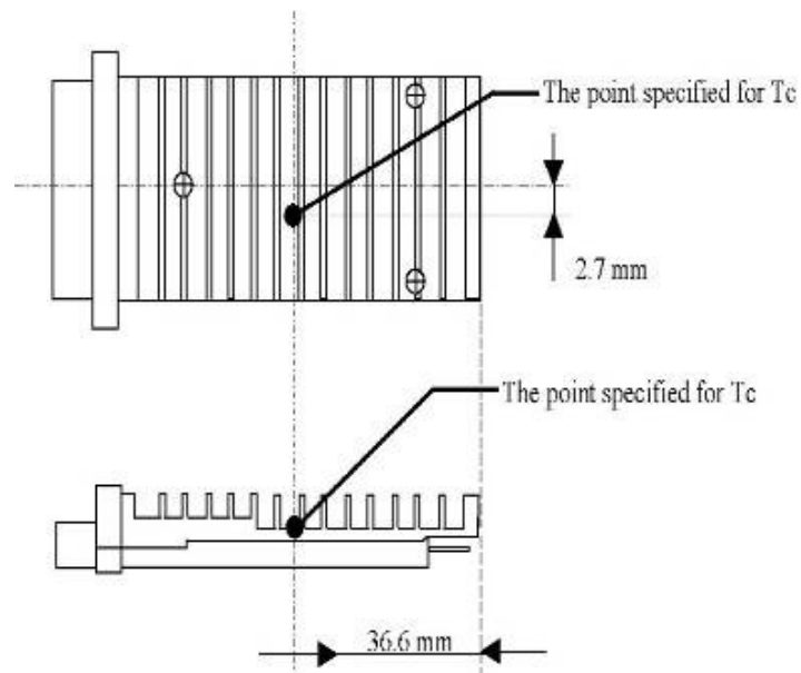
Figure 2 The Point Specified for Case Temperature ( T_c )
