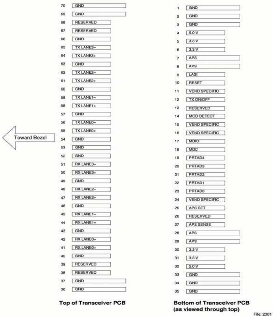
Fig 1-X2 Transponder Electrical Pad Layout
